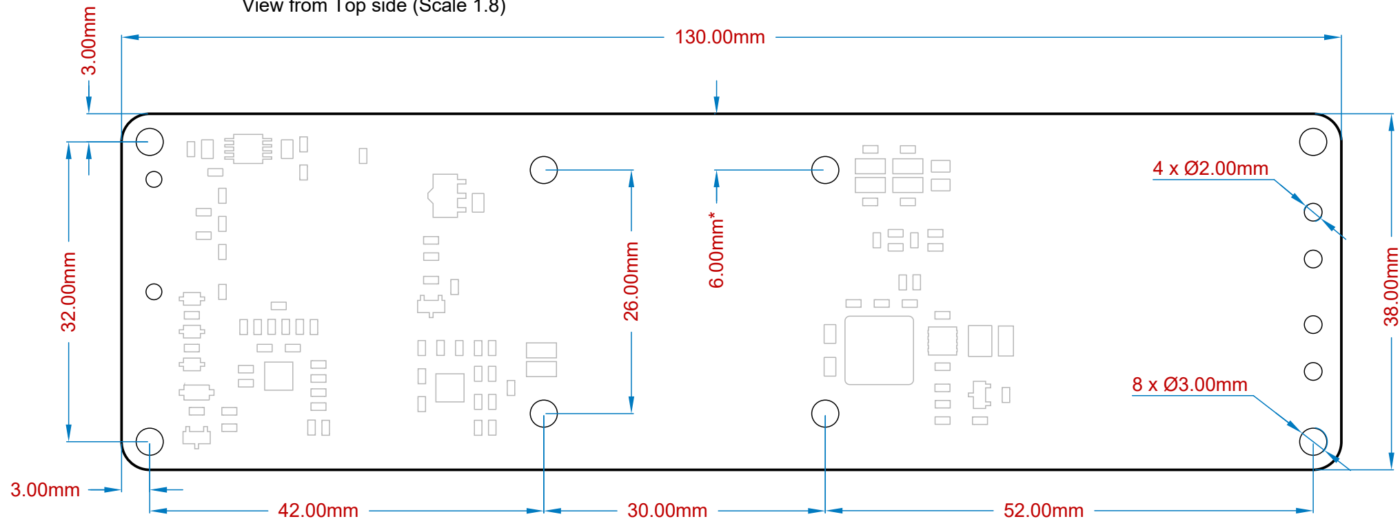
View from Top side (Scale 1.8)
