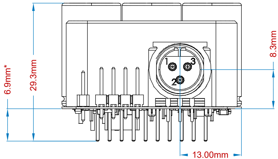
View from Left side (Scale 2:1)
