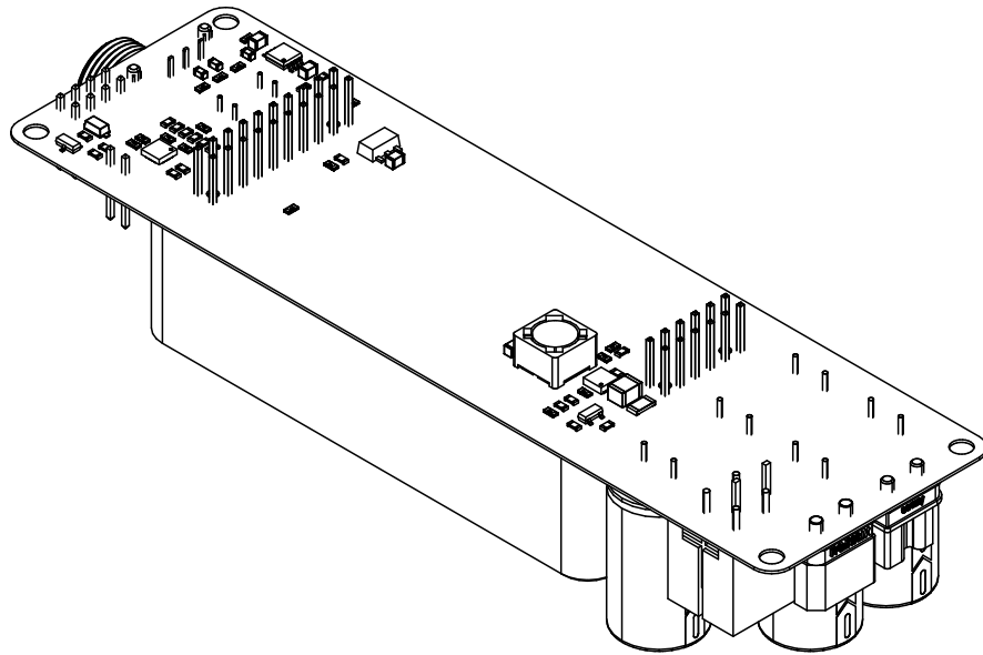
View from Front side (Scale 1:1)
